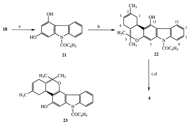
Scheme 3. (a) \text{BBr}_3/\text{CH}_2\text{Cl}_2 , 25 °C; (b) trans - p -menthadienol/HOTS/benzene, reflux; (c) KOH/DMSO then n - \text{C}_5\text{H}_{11}\text{Br} , 25 °C; (d) NaSPr/DMF, 120 °C.
