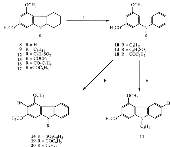
Scheme 2. (a) Chloranil, benzene, 80 °C; (b) Br 2 , HOAc, 25 °C.
